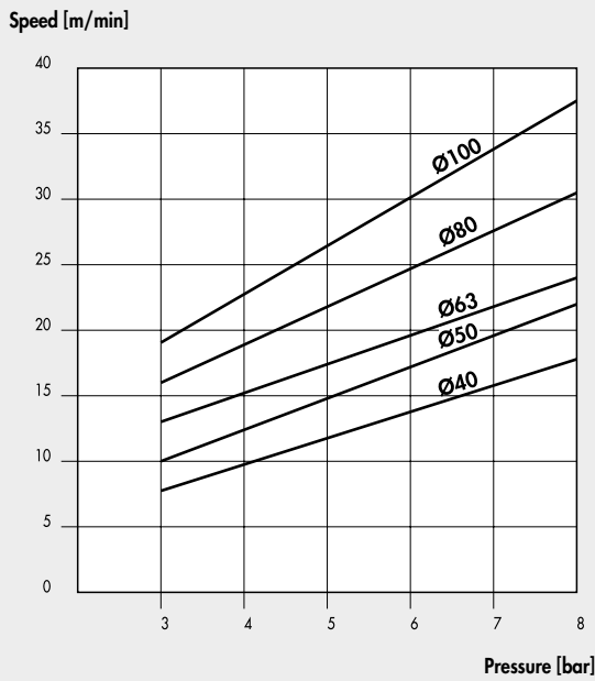
Ø40 BRK BRAKE WITH REGULATION, SKIP OR REGULATION + SKIP VALVE(S)
