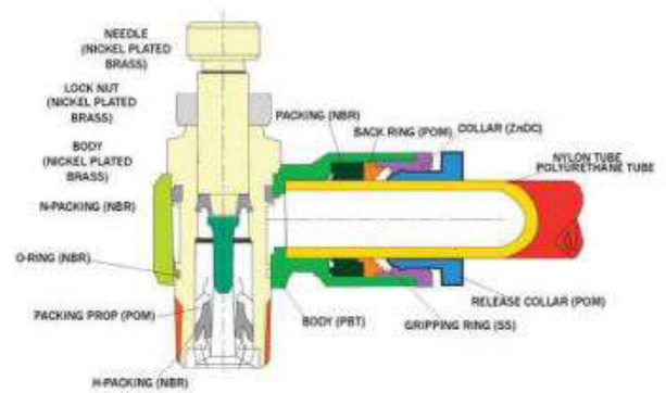
Figure 1.4 Diagram of Flow Controller
