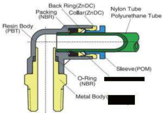
Figure 1.3 Diagram of Thread Fittings
